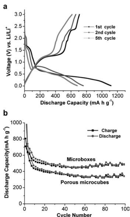
Figure 4. a) Discharge–charge voltage profiles and b) cycling performance of single-crystal MnS microboxes obtained at 800 °C and porous MnS microcubes obtained at 350 °C in the voltage window of 0.01–3.0 V vs. Li/Li + at a current density of 200 \text{ mA g}^{-1} .
